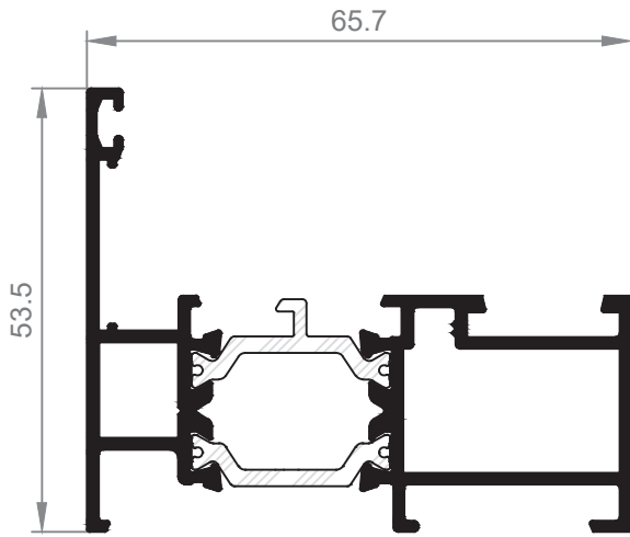
24001 Marco
