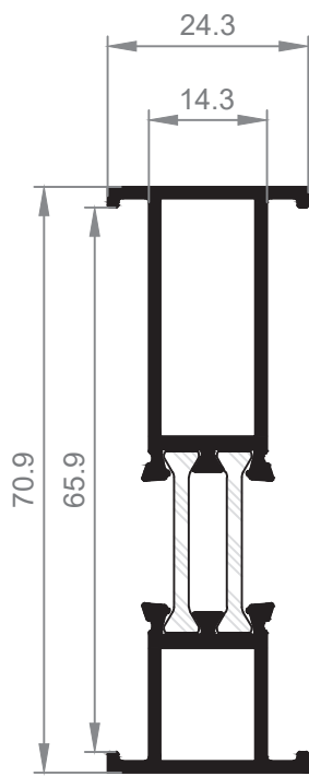
24000 Union Marcos
