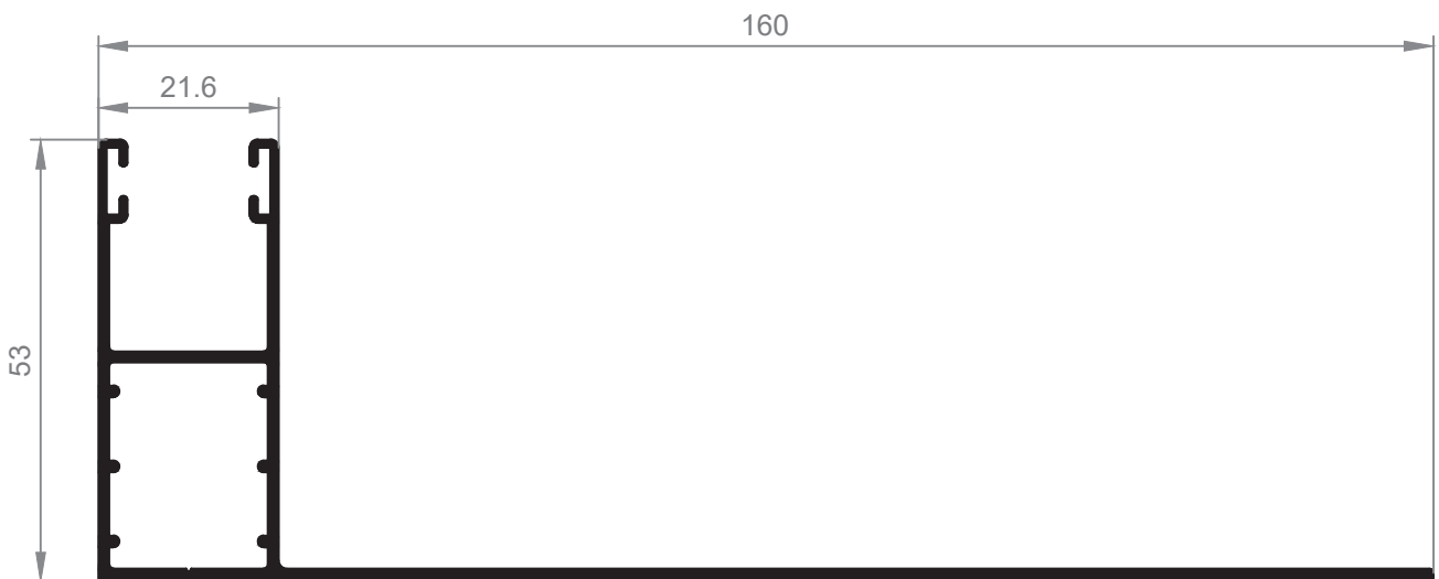
1196 Guia L 160mm Ala inferior
