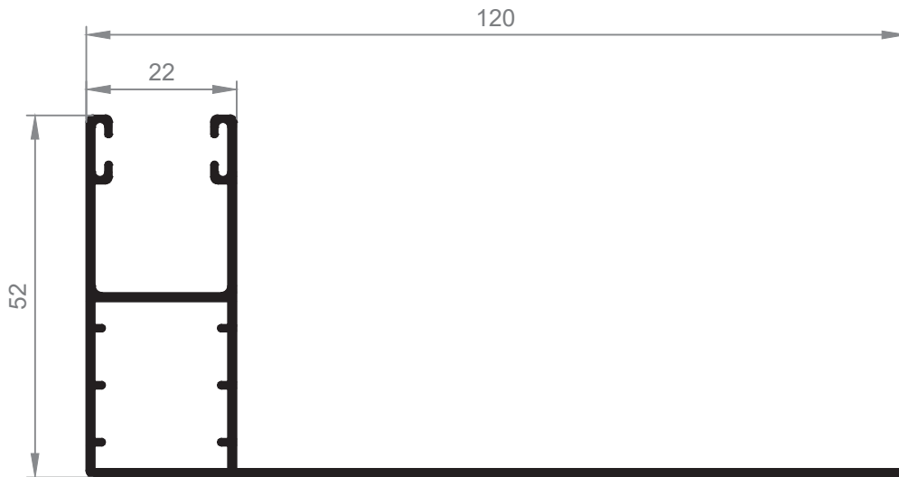
187 Guia Persiana 120mm "L" Ala Inferior
