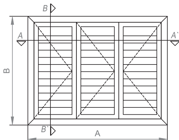
Contraventana practicable 3H perfil 214G
